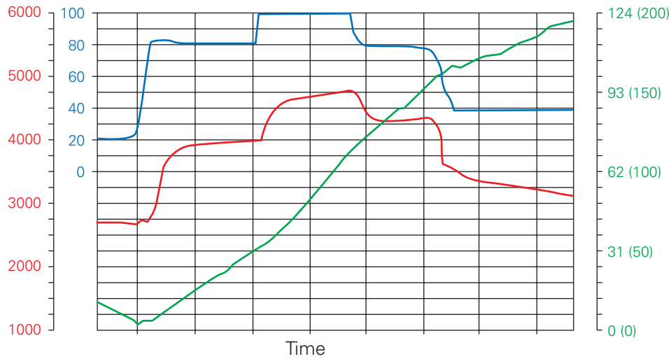
Engine Speed Response to Quick Changes in Accelerator Pedal Angle
