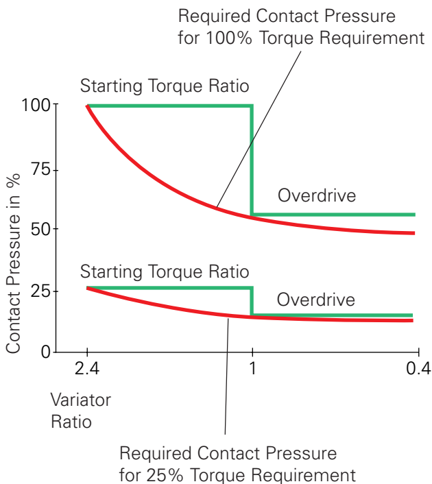
— Contact Pressure
